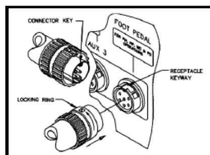
Figure 115. Foot Pedal Connection
