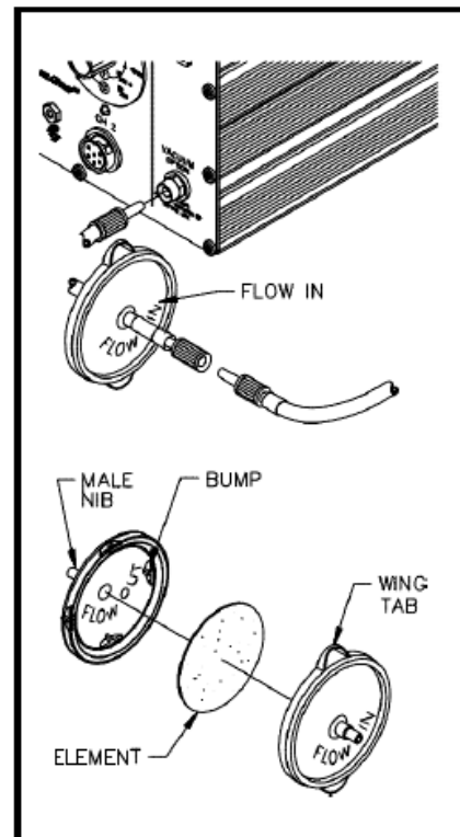
Figure 129. VisiFilter Element Replacement
