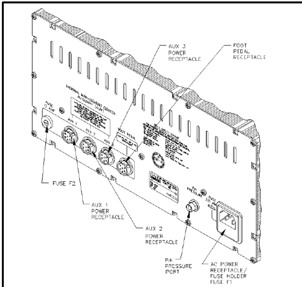
Figure 14. Rear Panel Parts I.D.
