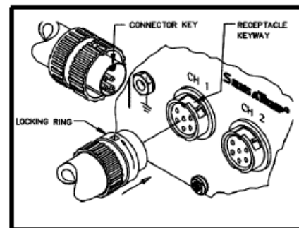
Figure 44. Handpiece Connection , TMC
