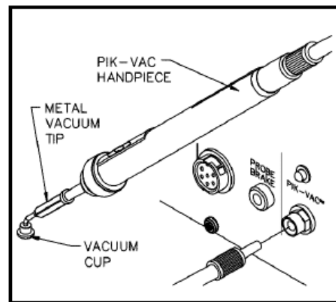
Figure 109. Pik-Vac Set-Up
