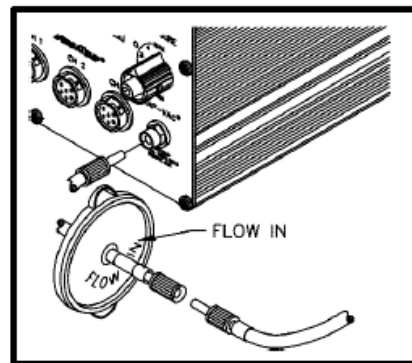
Figure 20. VisiFilter Preparation
