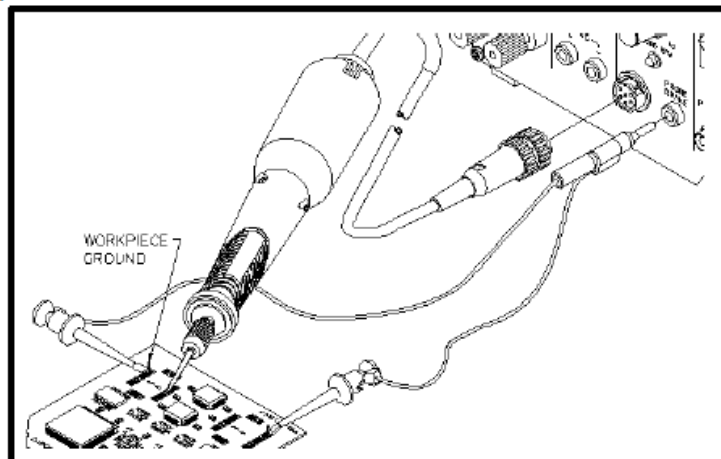
Figure 118. Workpiece Grounding
