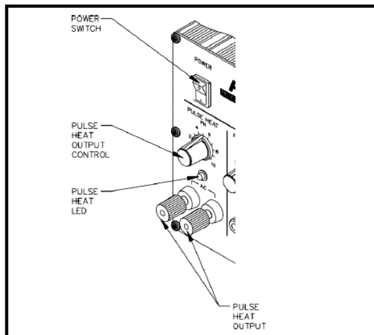
Figure 9. Pulse Heat Section
