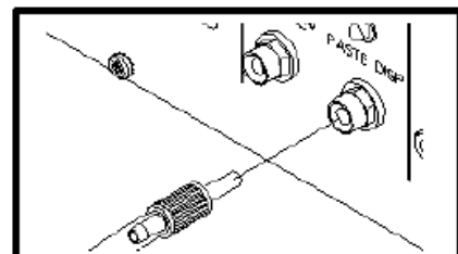
Figure 102. Paste Dispense Connection
