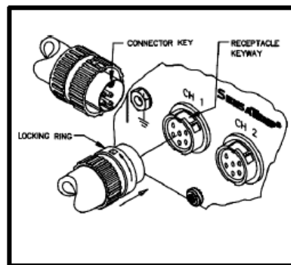
Figure 17. TMC Handpiece Connection
