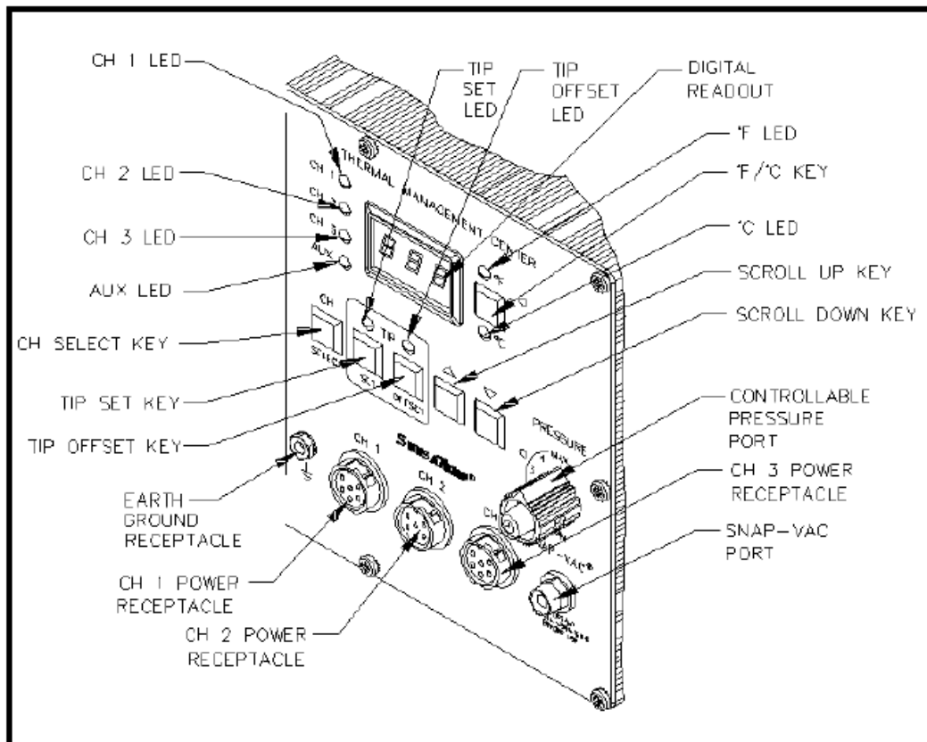
Figure 13. Thermal Management Center Parts I.D.
