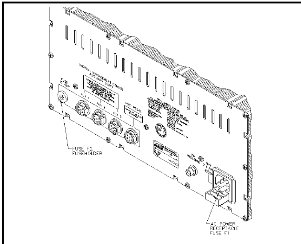
Figure 131. Power Source Rear Panel
