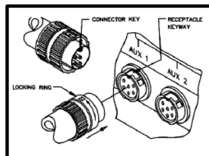
Figure 99. Aux. Foot Pedal Connection
