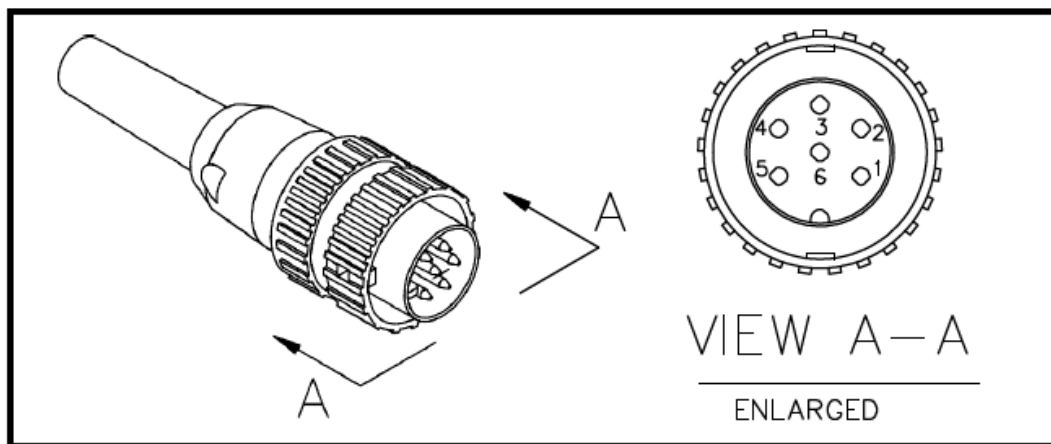
Figure 130. Handpiece Connector Plug
