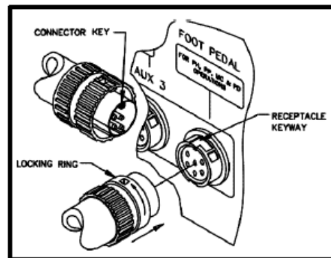
Figure 121. Foot Pedal Connection
