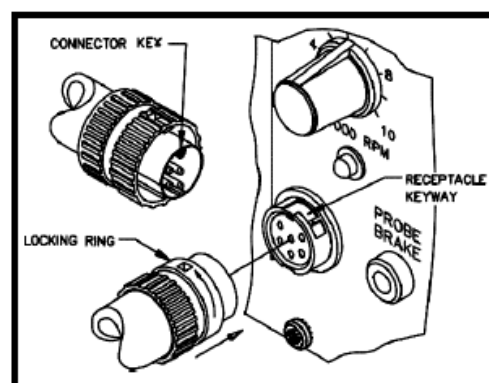
Figure 112. MicroChine Attachment
