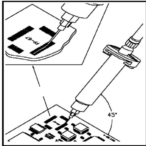
Figure 107. Paste Dispensing
