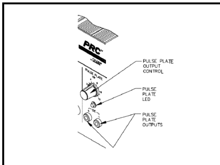
Figure 10. Pulse Plate Section
