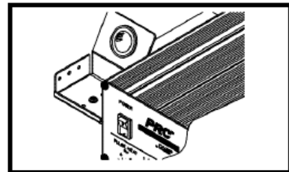
Figure 100. Dispenser Cubby Mounting
