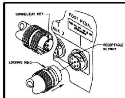
Figure 97. Foot Pedal Connection
