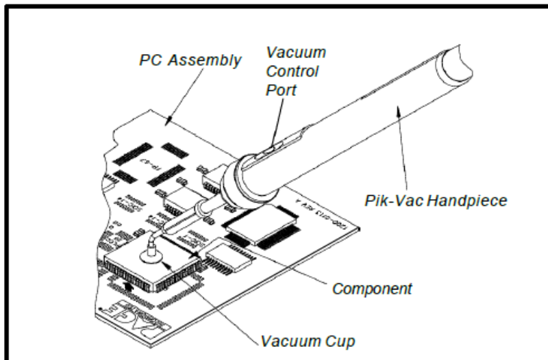
Figure 111. Pik-Vac Operation
