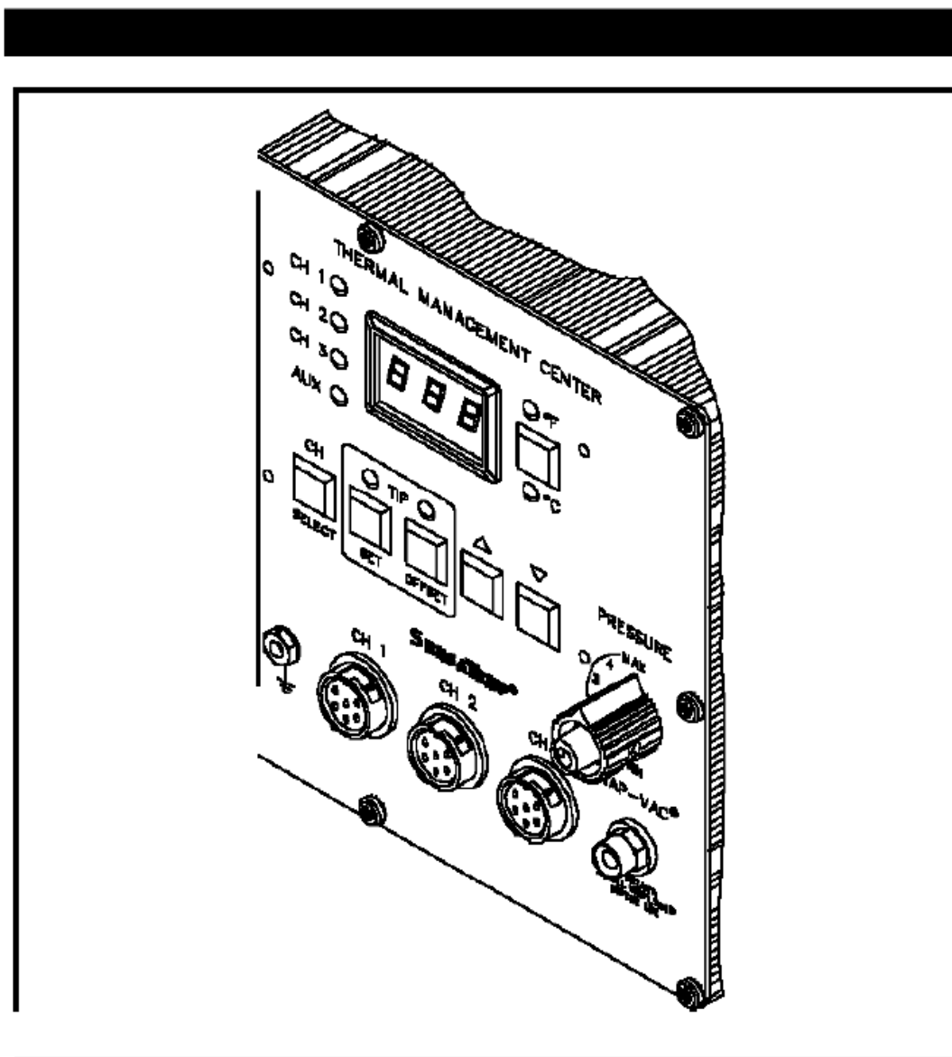
Figure 6 Thermal ManagementCenter
