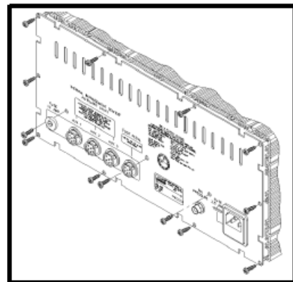
Figure 73. Rear Panel Removal
