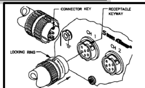
Figure 21. Handpiece Connection to TMC
