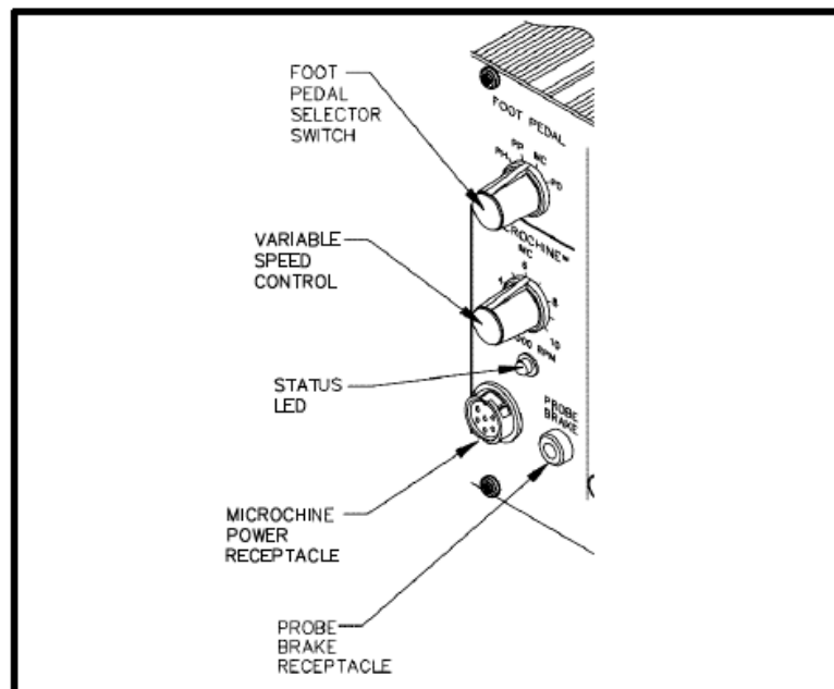
Figure 11. MicroChine Section
