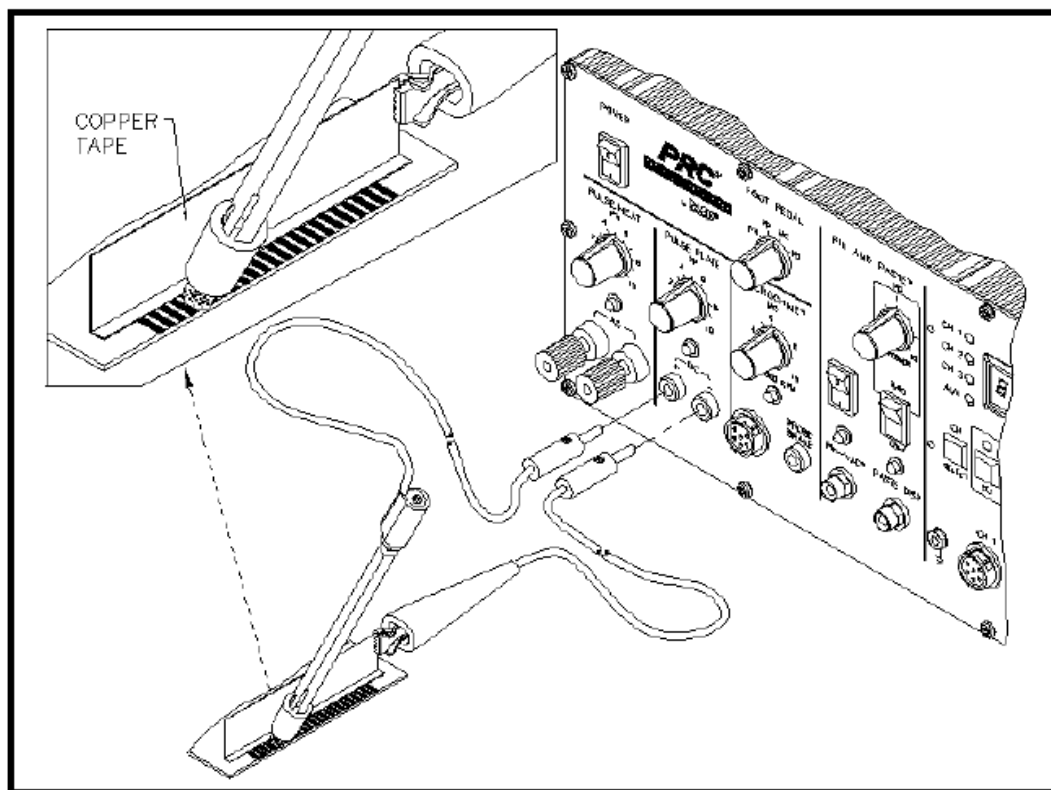
Figure 122. Pulse Plate Set-Up
