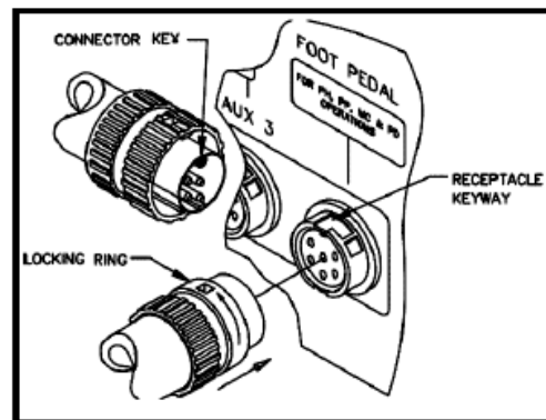
Figure 123. Foot Pedal Connection
